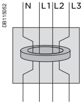
With a Vigi module, the deviation of the N and L3 bars required to pass through the toroid results in higher power losses compared to those of the L1 and L2 bars.
