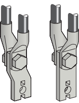
Mounting detail: 2 cables with lugs.
